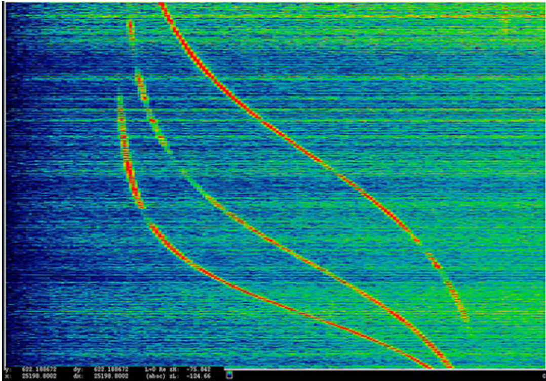
“ANARCHIST: Power Spectrum Display of Doppler Tracks from a Satellite (Intercepted May 27, 2009), 2016.” by Laura Poitras (b. 1964). Pigmented inkjet print mounted on aluminum, 45 × 64 3/4 inches. Courtesy the artist.
